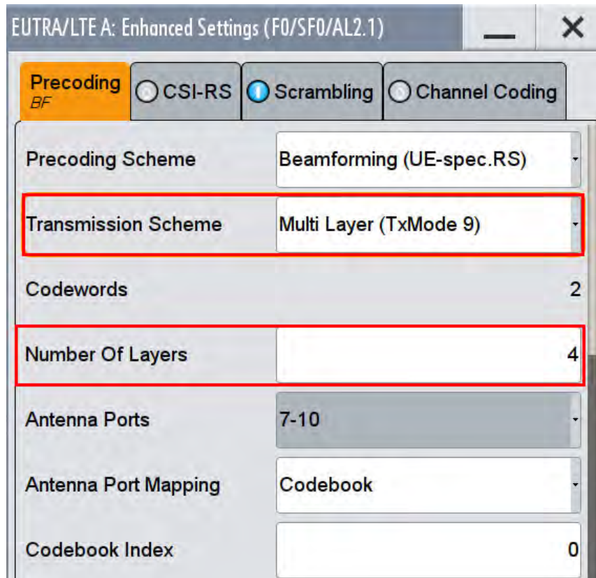
Figure 2-17: SMW: TM9 in the enhanced settings of the subframe, here with four layers
