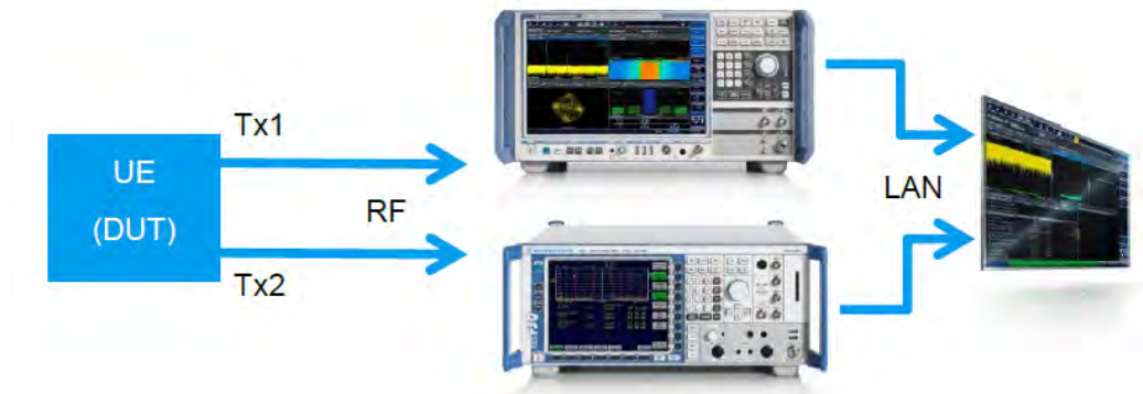
Figure 2-32: Test setup for measuring a 2x2 uplink MIMO signal
