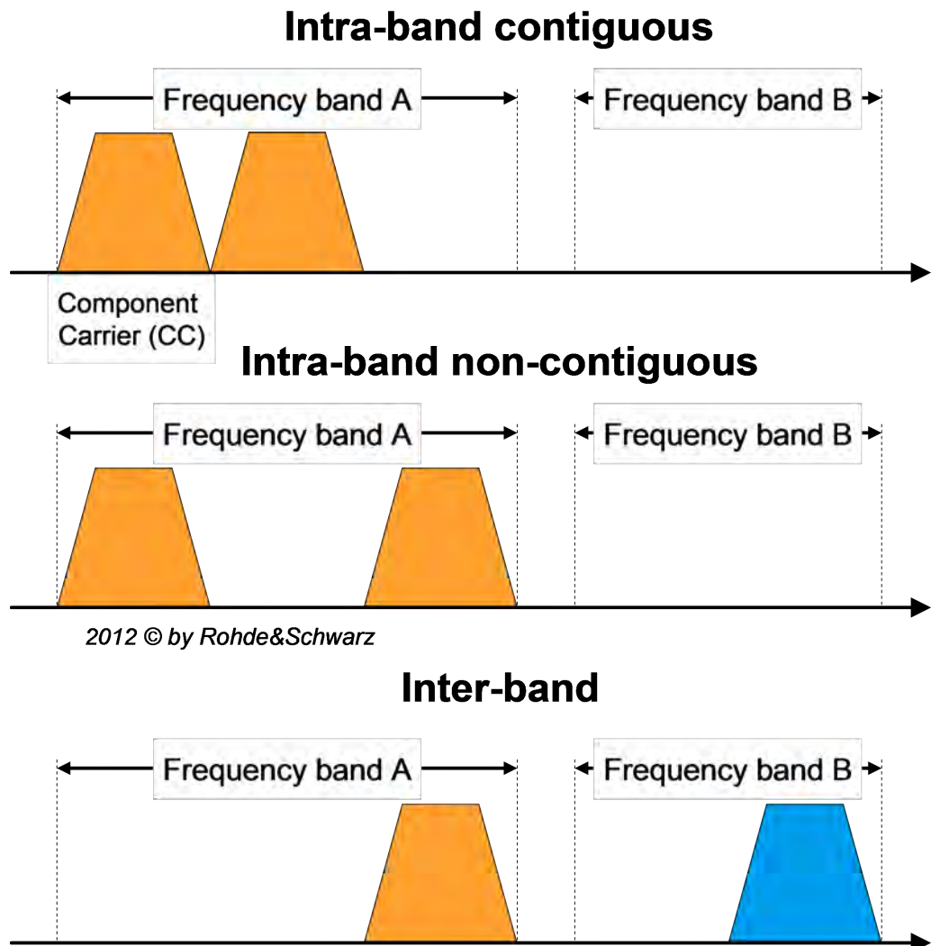
Figure 2-2: Modes of carrier aggregation
