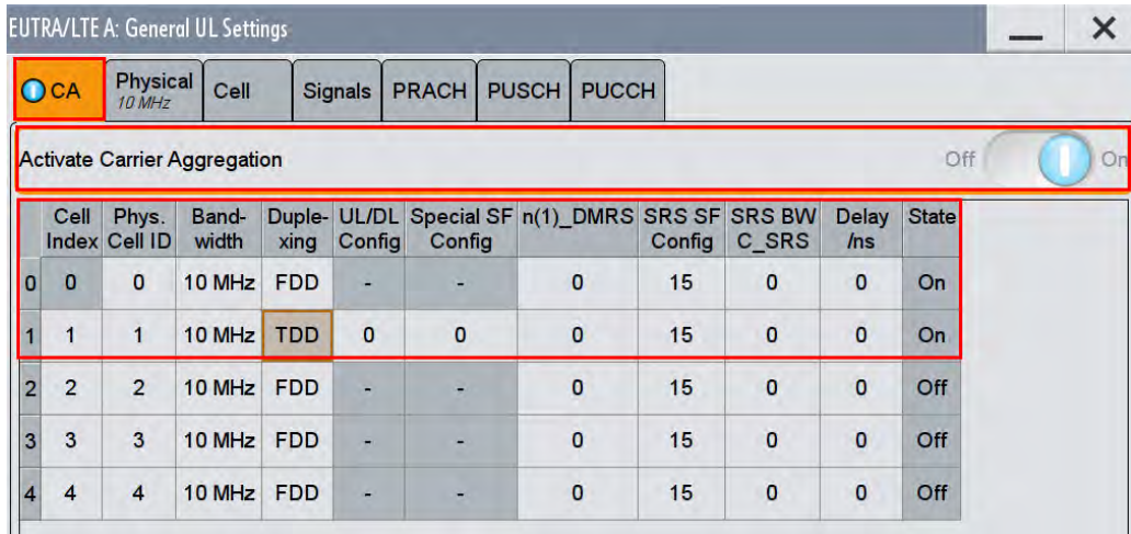
Figure 2-12: SMW: UL Carrier Aggregation
