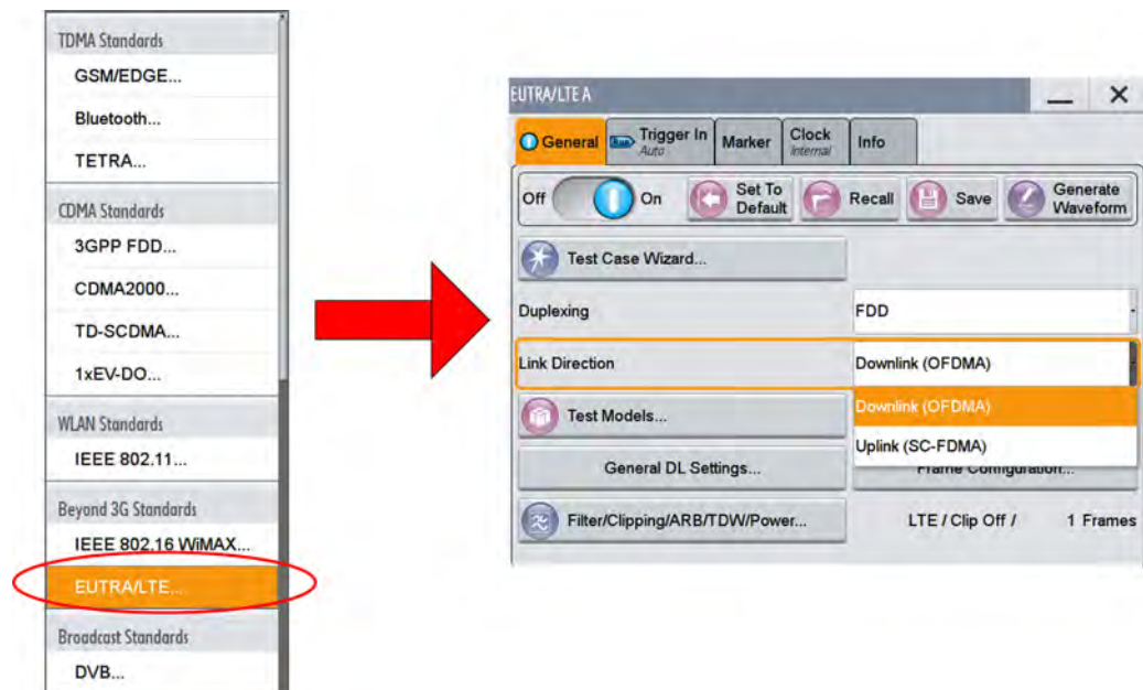
Figure 2-8: Start of the LTE standard and Link Direction.
