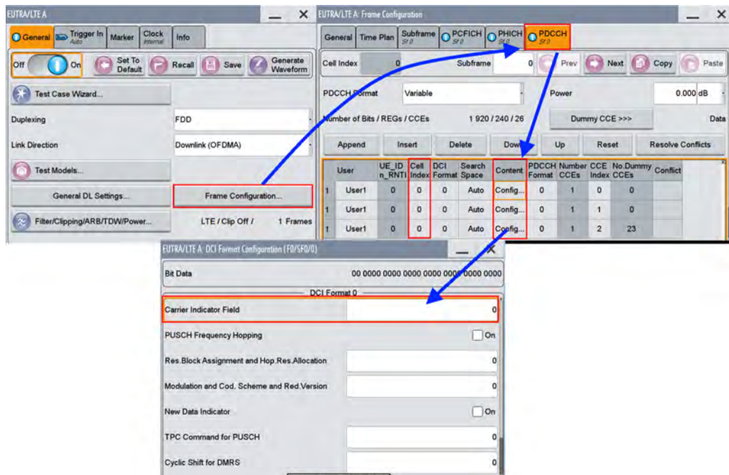
Figure 2-11: Configuring the content of the CFI field for each user
