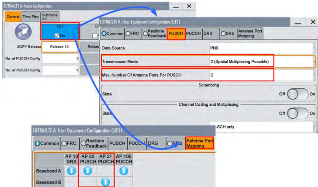
Figure 2-19: The Transmission Mode 2 enables Spatial Multiplexing with up to four antennas (example 2 antennas)
