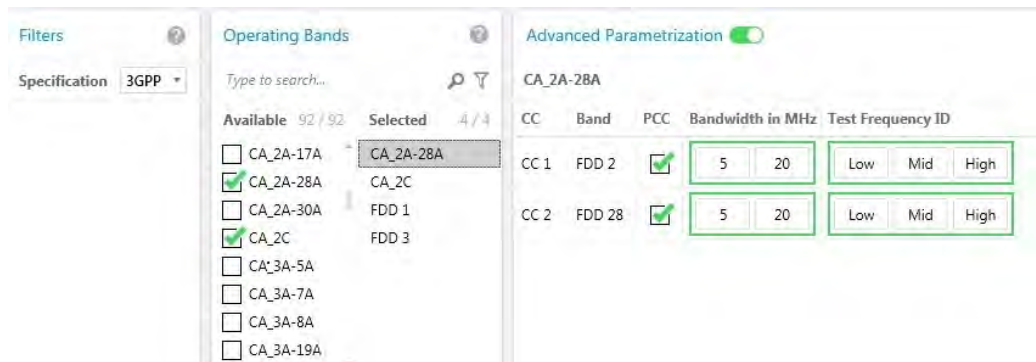
Figure 2-47: CA band combinations in Contest
