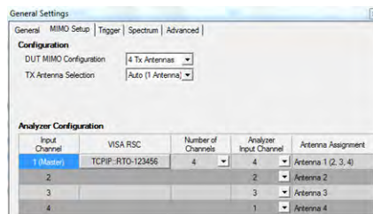
Figure 2-22: Using the RTO for MIMO measurements
