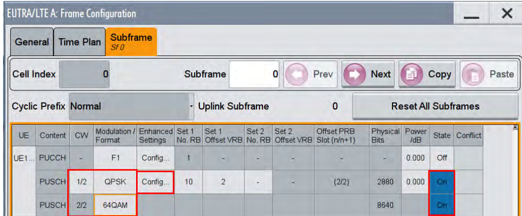
Figure 2-20: Setting the two independent codewords.
