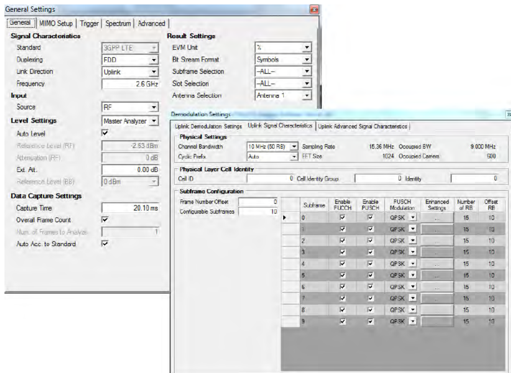
Figure 2-30: Demodulation settings for enhanced SC-FDMA
