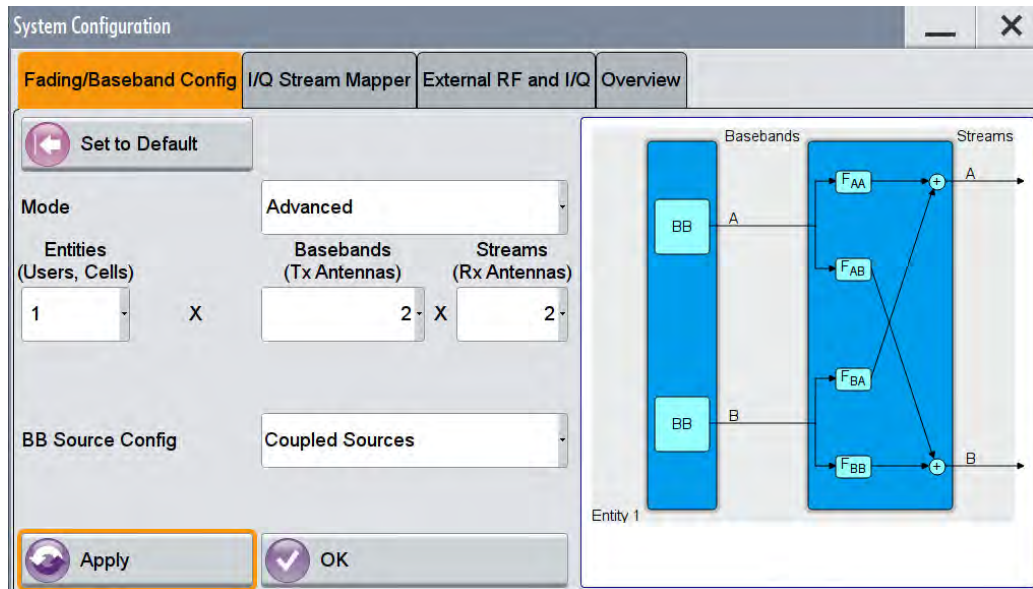
Figure 2-18: The system configuration for a 2x2 Uplink MIMO is 1 x 2 x 2
