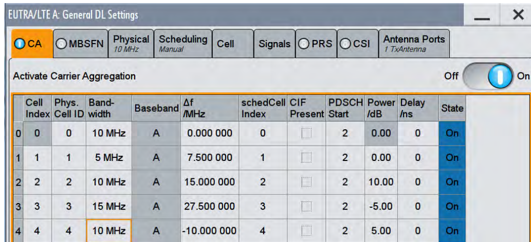
Figure 2-9: Carrier aggregation settings with up to five carriers in one baseband (SMW-K85). The carrier with cell index 0 is the Primary Component Carrier (PCC)
