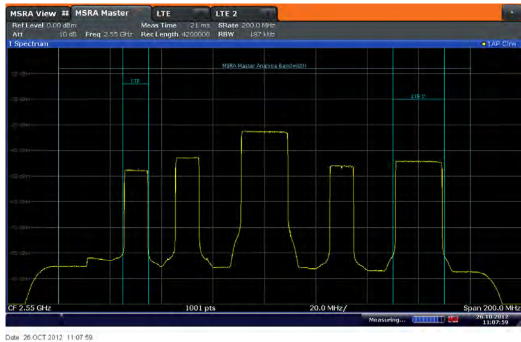
Figure 2-26: MSRA master view of a five component LTE-A carrier aggregation signal
