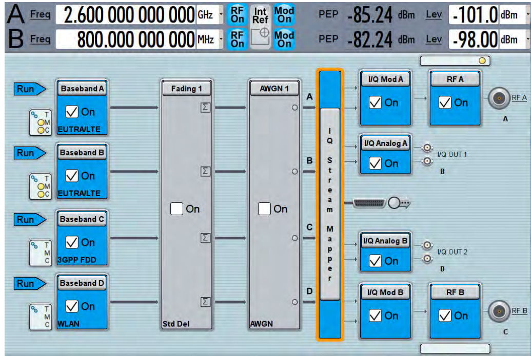
Figure 2-7: SMW example with four different signals
