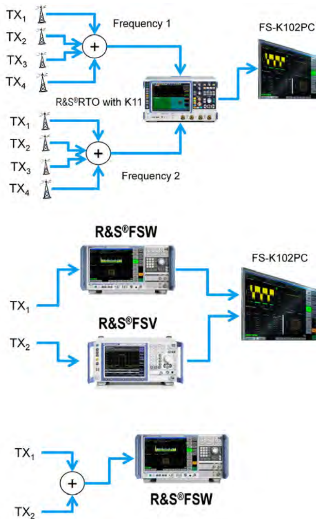
Figure 2-28: different setups measuring TAE for carrier aggregation
