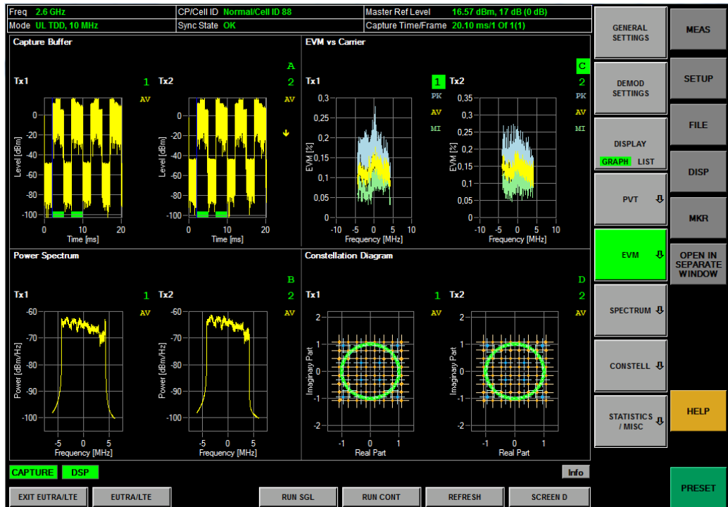
Figure 2-35: Power versus time / frequency measurements, EVM measurements and constellation diagram for each Tx antenna summarized in the multiple screen view
