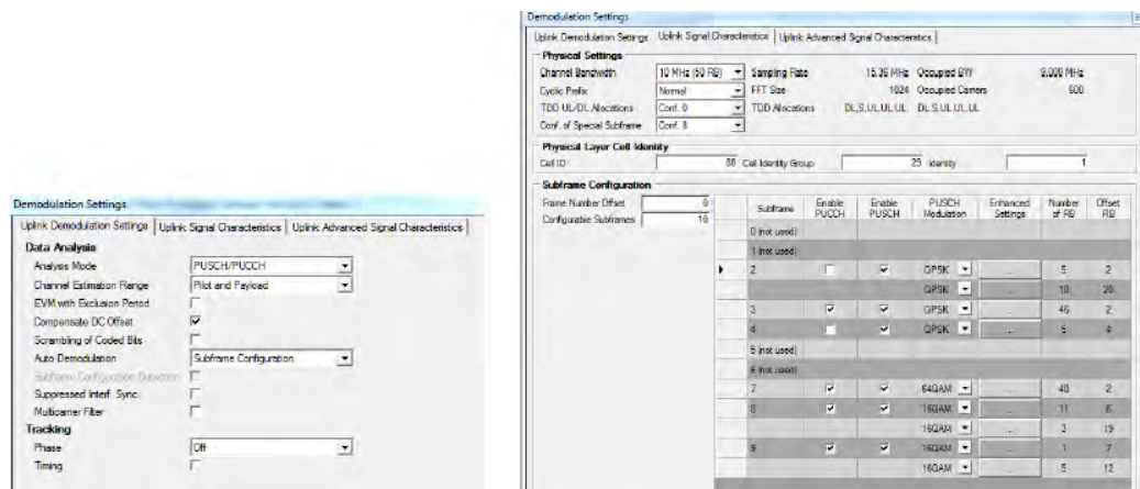
Figure 2-34: General settings to measure an uplink 2x2 MIMO LTE TDD signal (10 MHz)
