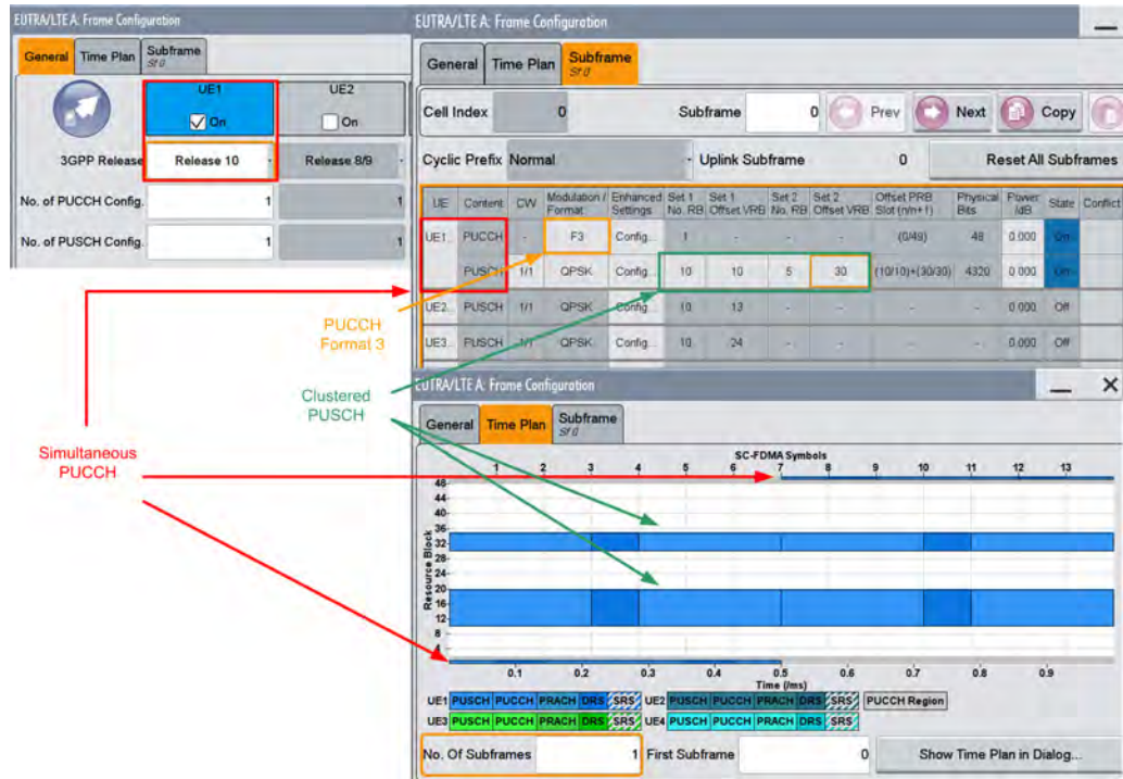
Figure 2-15: Configuring Clustered PUSCH and simultaneous PUCCH/PUSCH
