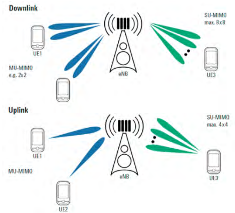
Figure 2-5: Supported transmit layers in LTE-Advanced
