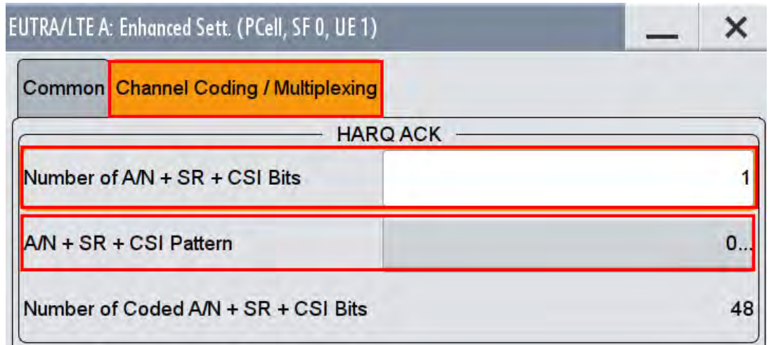
Figure 2-14: SMW: Set the bits to transmit in PUCCH format 3
