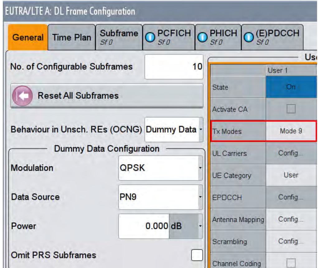
Figure 2-16: SMW: TM9 settings in the general DL frame configuration
