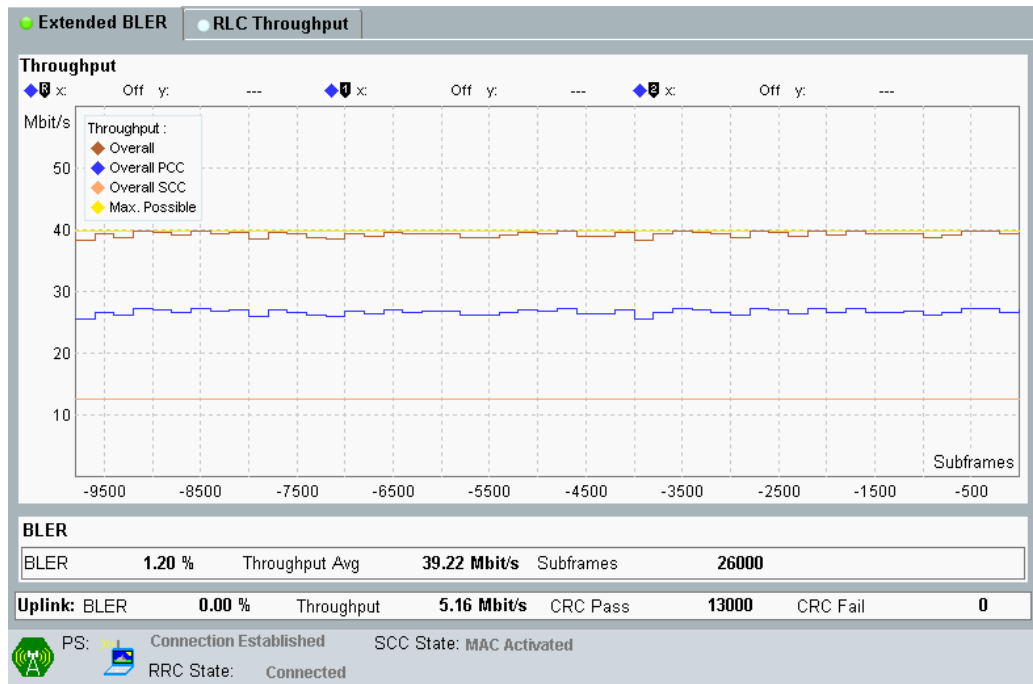
Figure 2-43: LTE RX measurement for Carrier Aggregation. The throughput for both CCs and the overall throughput are displayed.
