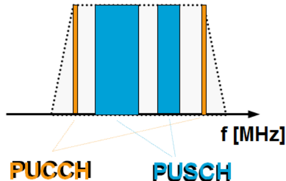
Figure 2-3: Simultaneous PUCCH/PUSCH and clustered uplink operation
