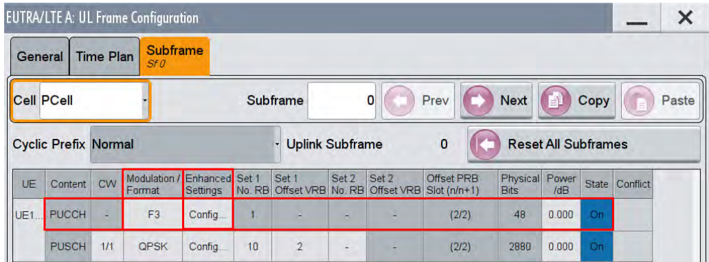
Figure 2-13: SMW PUCCH format 3
