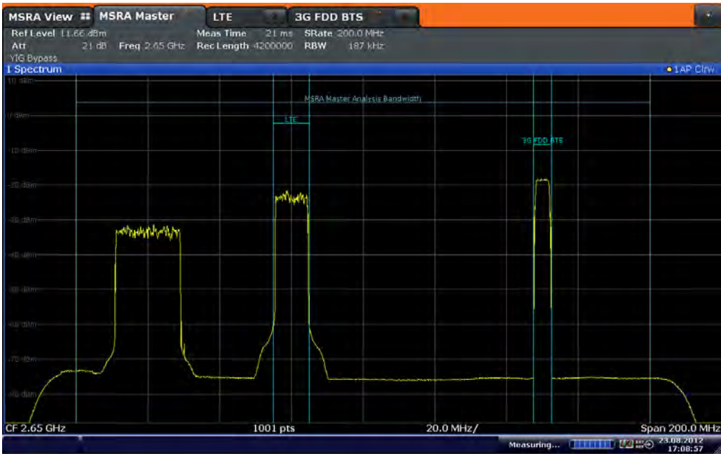
Figure 2-24: FSW MSRA spectrum measurement of a multi-technology and multi-carrier signal
