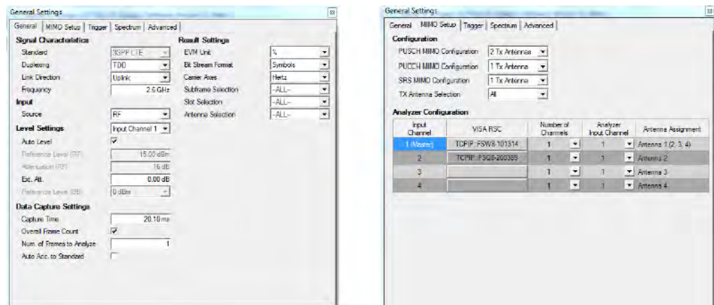
Figure 2-33: General settings to measure an uplink 2x2 MIMO LTE TDD signal (10 MHz)
